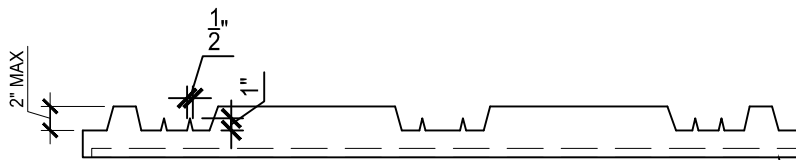
FORM LINER SECTION VIEW: A
