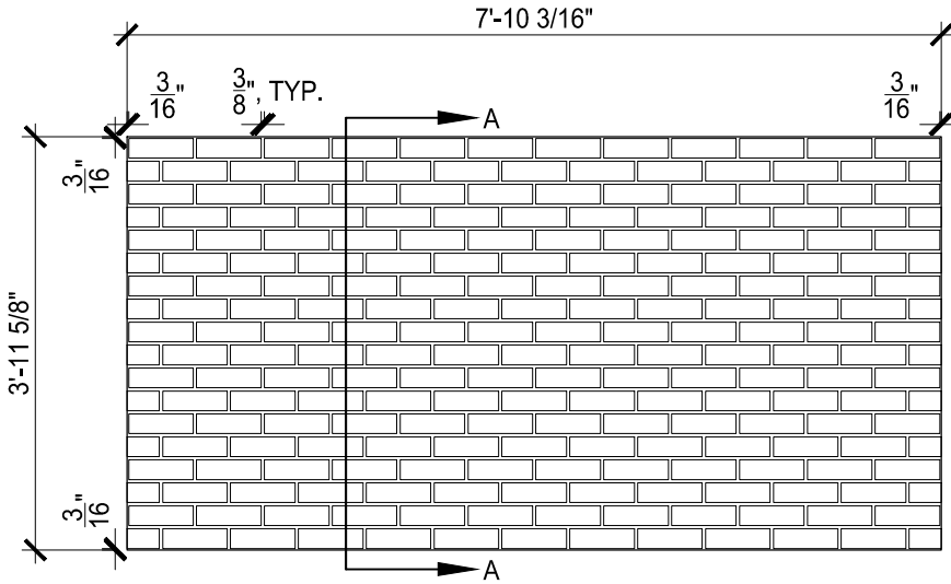
CONCRETE ELEVATION VIEW
