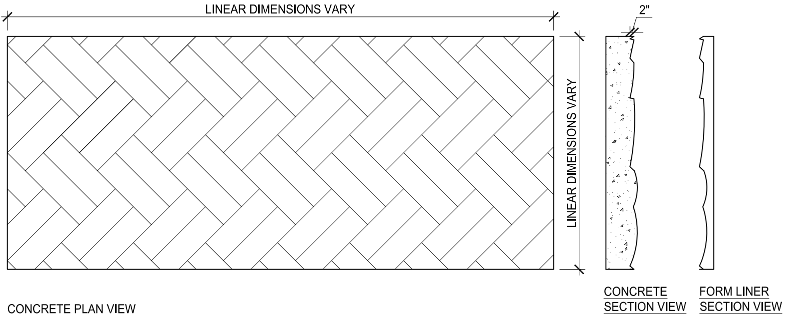
CONCRETE PLAN VIEW
