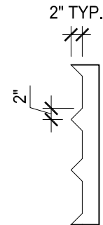
FORM LINER SECTION VIEW: A
