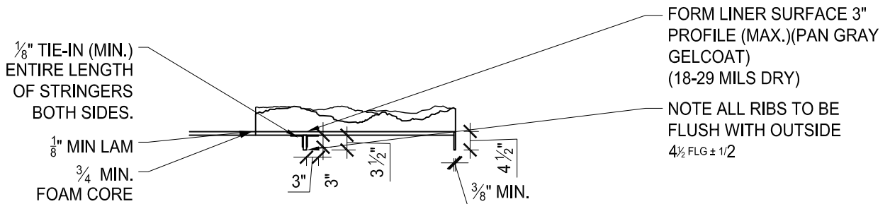
SECTION - A
