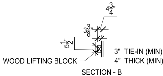
SECTION - B
